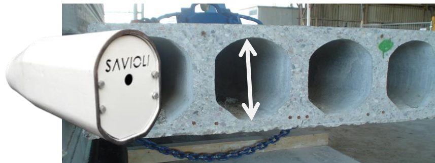
Excellent void forming into the slab
