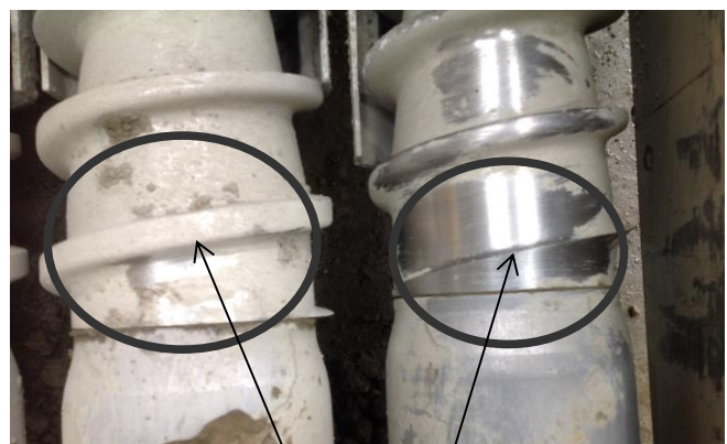
Slow wear of the spiral pitch
